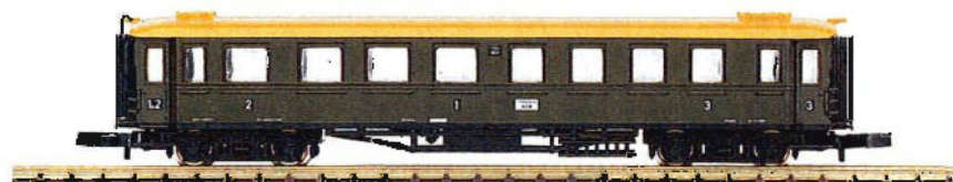
I 87940 Württemberg Express Train Passenger Car. Prototype: Royal Württemberg State Railways (K.W.St.F.) type ABCGÜ. 1st/2nd/3rd class. Model: Length over buffers 88 mm / 3-15/32".
