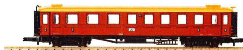
I 87950 Württemberg Express Train Passenger Car. Type BCCü. 2nd and 3rd class. Length over buffers 88 mm (3-15/32").
