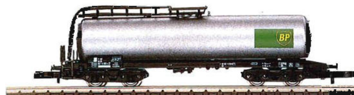
8614 Oil Tank Car. Privately owned by German BP, Inc. Length over buffers 40 mm (1-9/16").
